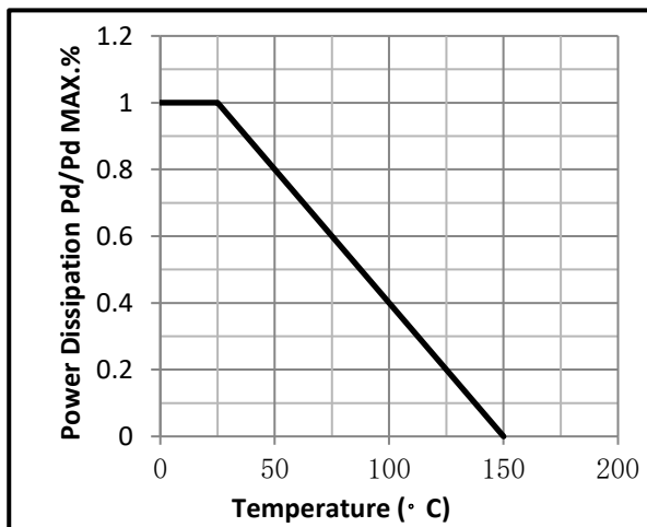
Fig.3 Power Dissipation
